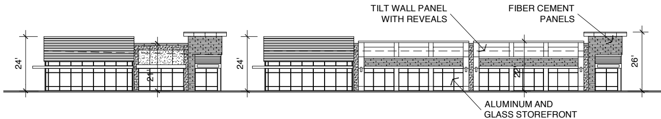
WEST ELEVATION
